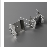
mounting plate U9 spring /plastic bag [2pcs] index: V4620019S
