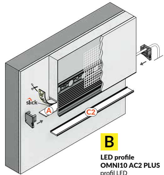
A LED profile OMNI10 AC2 profil LED OMNI10 AC2
